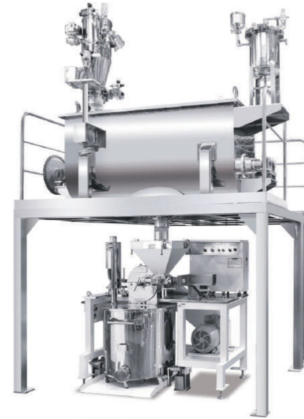
POWDER MIXING PLANT
